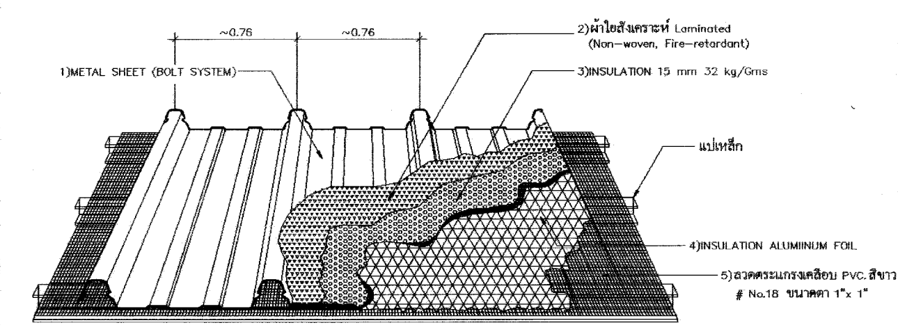
INSTALLATION ROOF + HEAT GUARD + WIRE MESH PVC.
